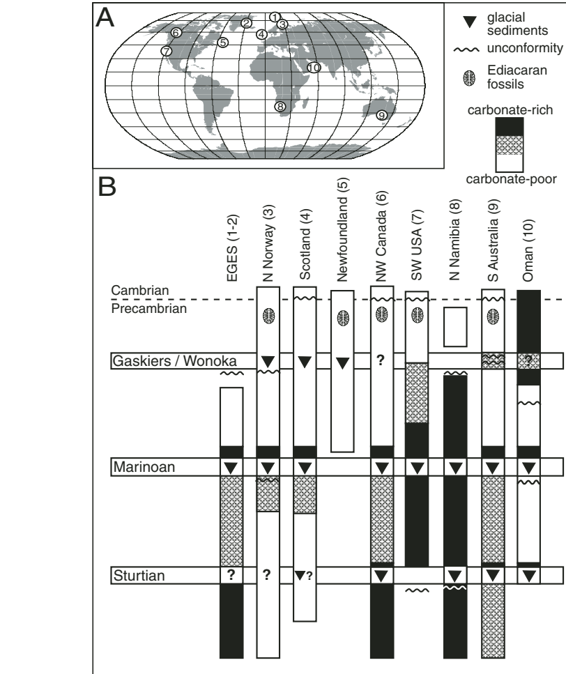
Figure 1. (A) Present-day locations of the Neoproterozoic successions discussed in this paper. (B) Schematic profiles of the successions from (A), showing their stratigraphic range, simplified lithologies, distribution of glacial deposits, and occurrence of Ediacaran fossils. See text for references. EGES—East Greenland-East Svalbard platform.
